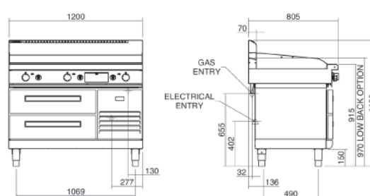
GP8120G-RB REFRIGERATED BASE
