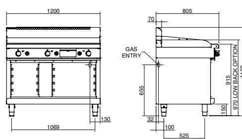
GP8120G-CB CABINET BASE
