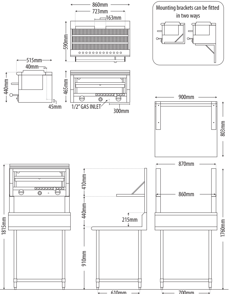
S86 pictured mounted on optional RCS21004 stand
