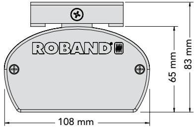
Dimensions for standard quartz lamps and fluorescent lighting assemblies (HQ & HF).
