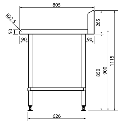
WALDORF SIDE ELEVATION
