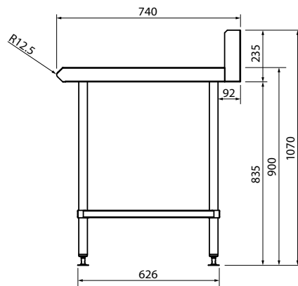
BLUE SEAL SIDE ELEVATION
