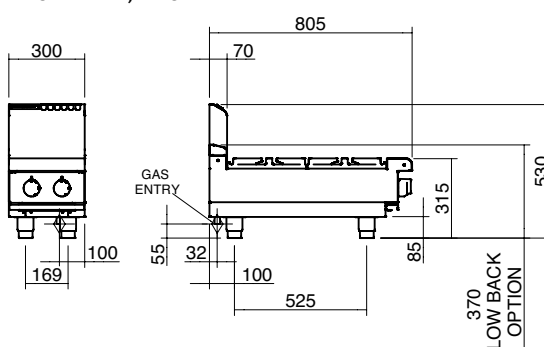
RN8200G-B, RN8203G-B
